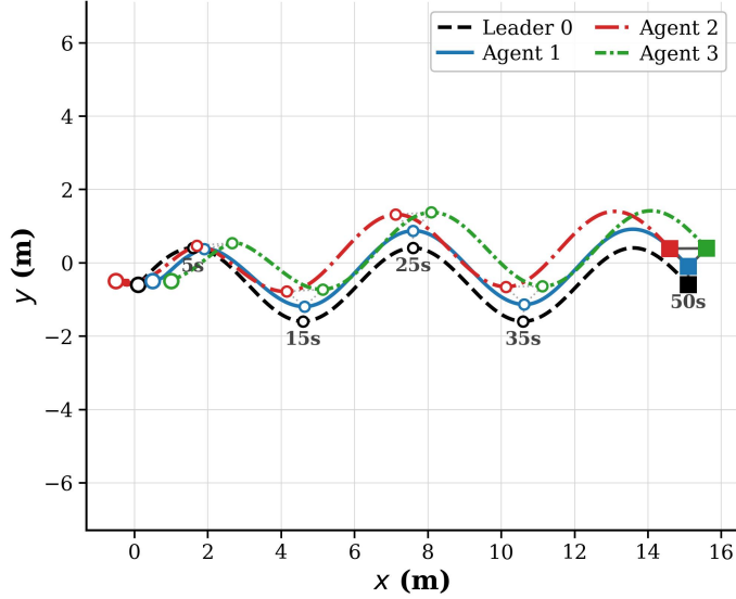
(b) Trajectories of relative motion of the WMRs, with the rigid formation edges redrawn at five time snapshots (5, 15, 25, 35, 50 s) to show the formation actually being carried along the path rather than only its start and end.
