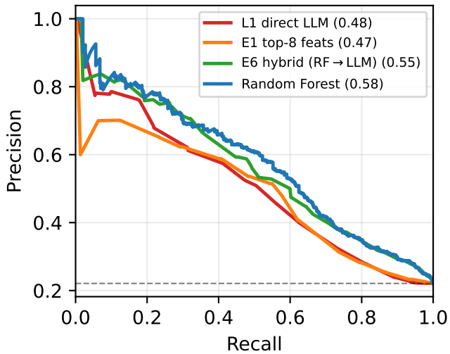
Precision-Recall (AP in legend)
