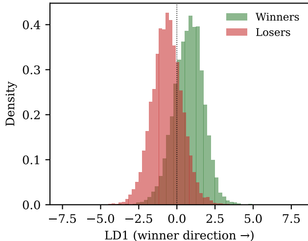
(a) Distribution along LD1
