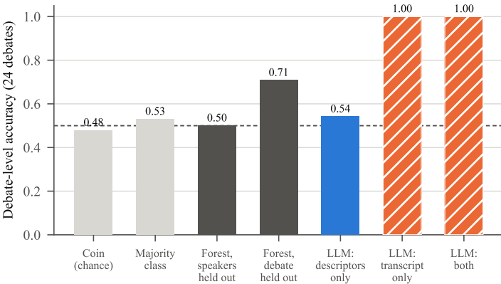
(a) Contaminated conditions look best
