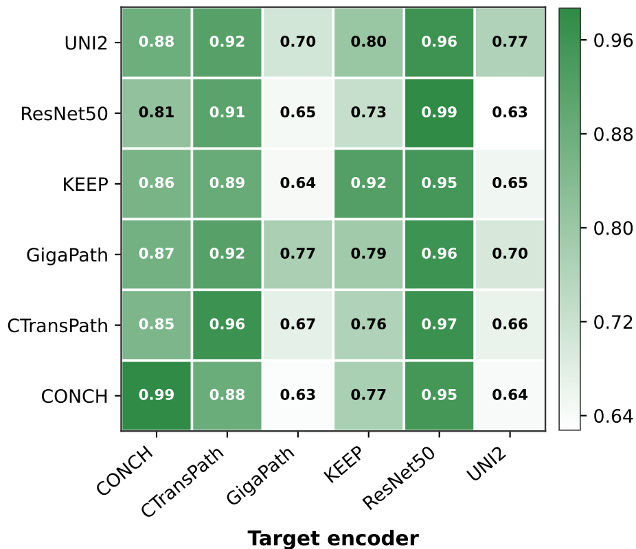
Cosine to real target
