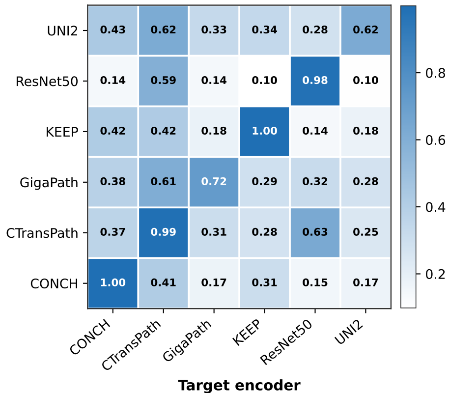
Retrieval Recall@1
