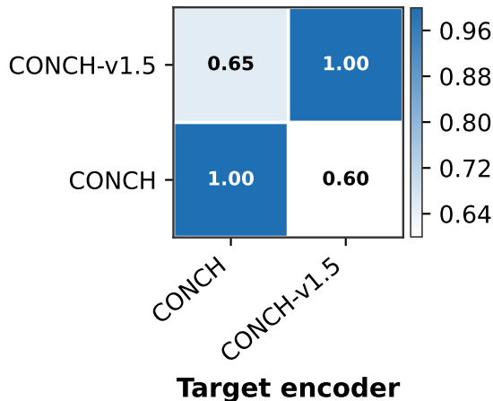
Retrieval Recall@1
