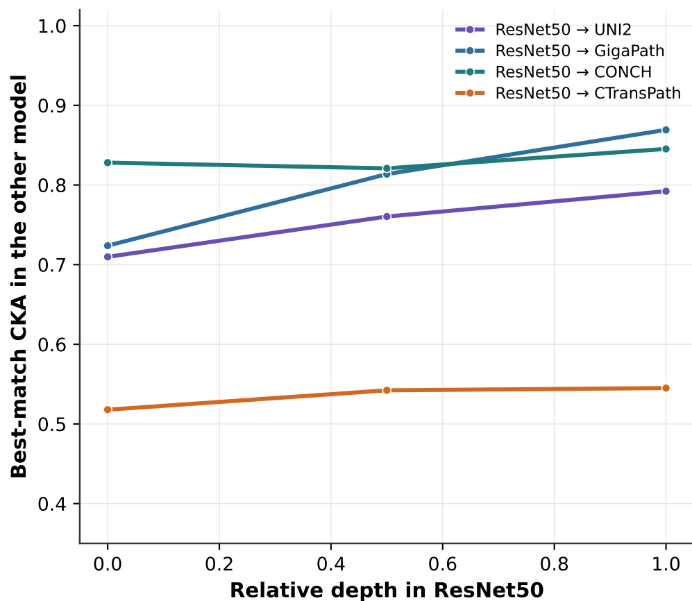
ResNet50's alignment across depth
