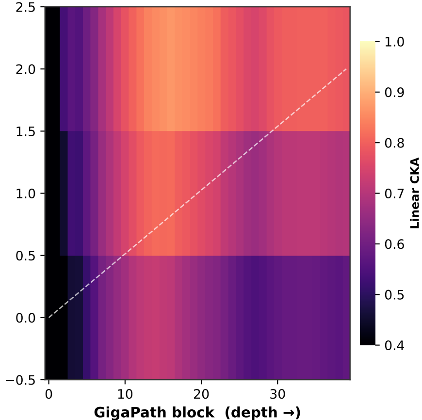
Block-by-block CKA
