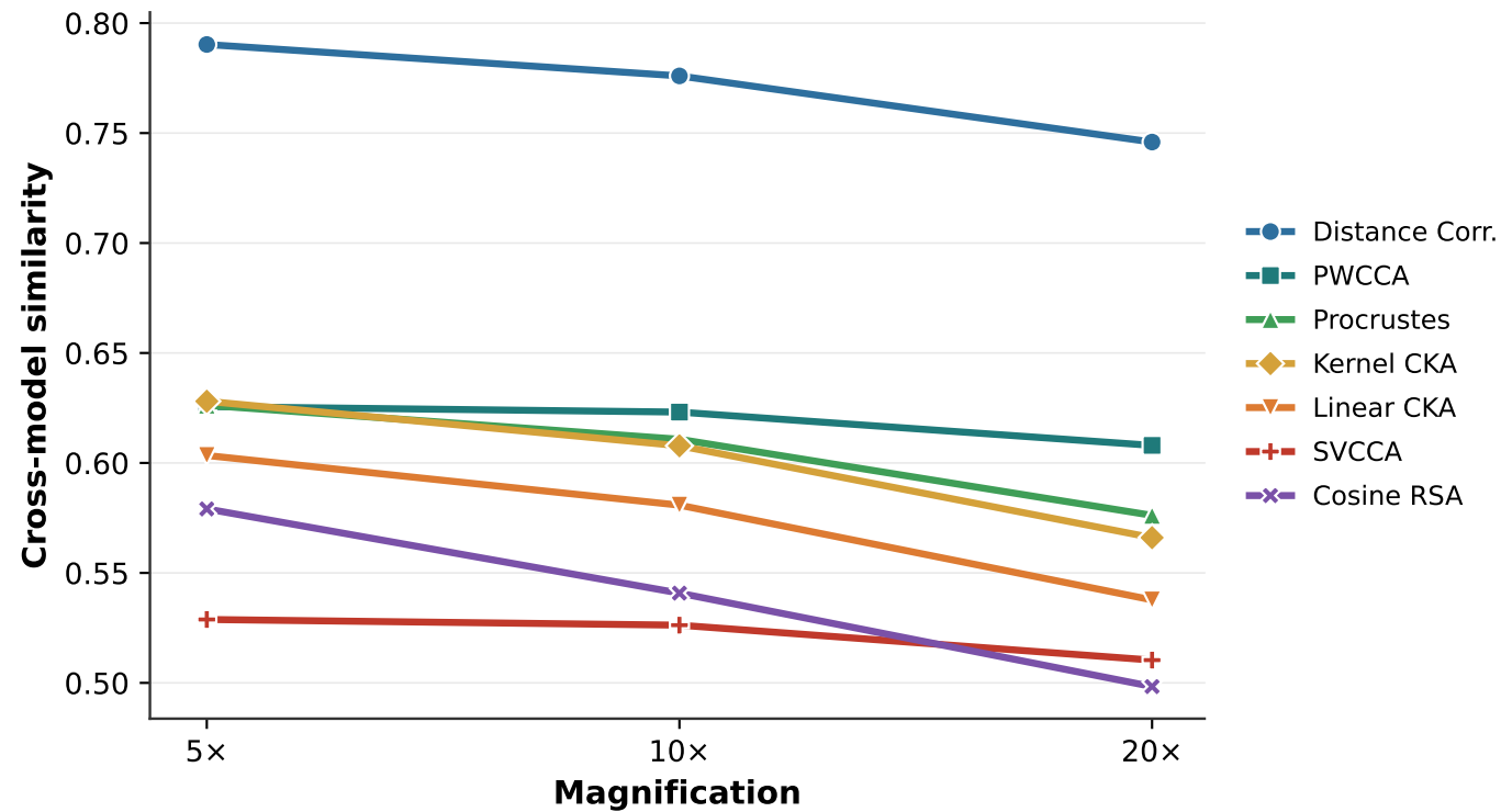
Agreement vs magnification — cptac_benchmark_256px
