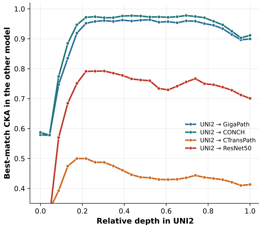
UNI2's alignment across depth
