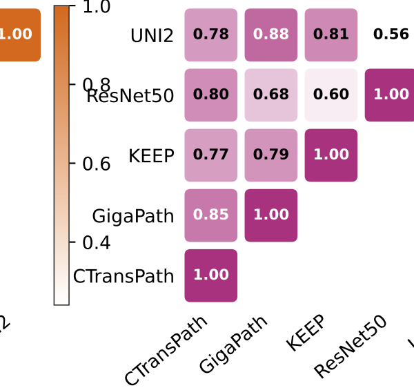
Distance Correlation
