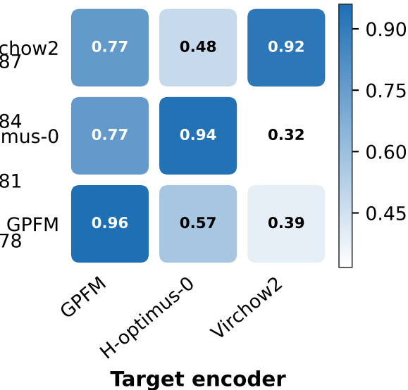
Retrieval Recall@1
