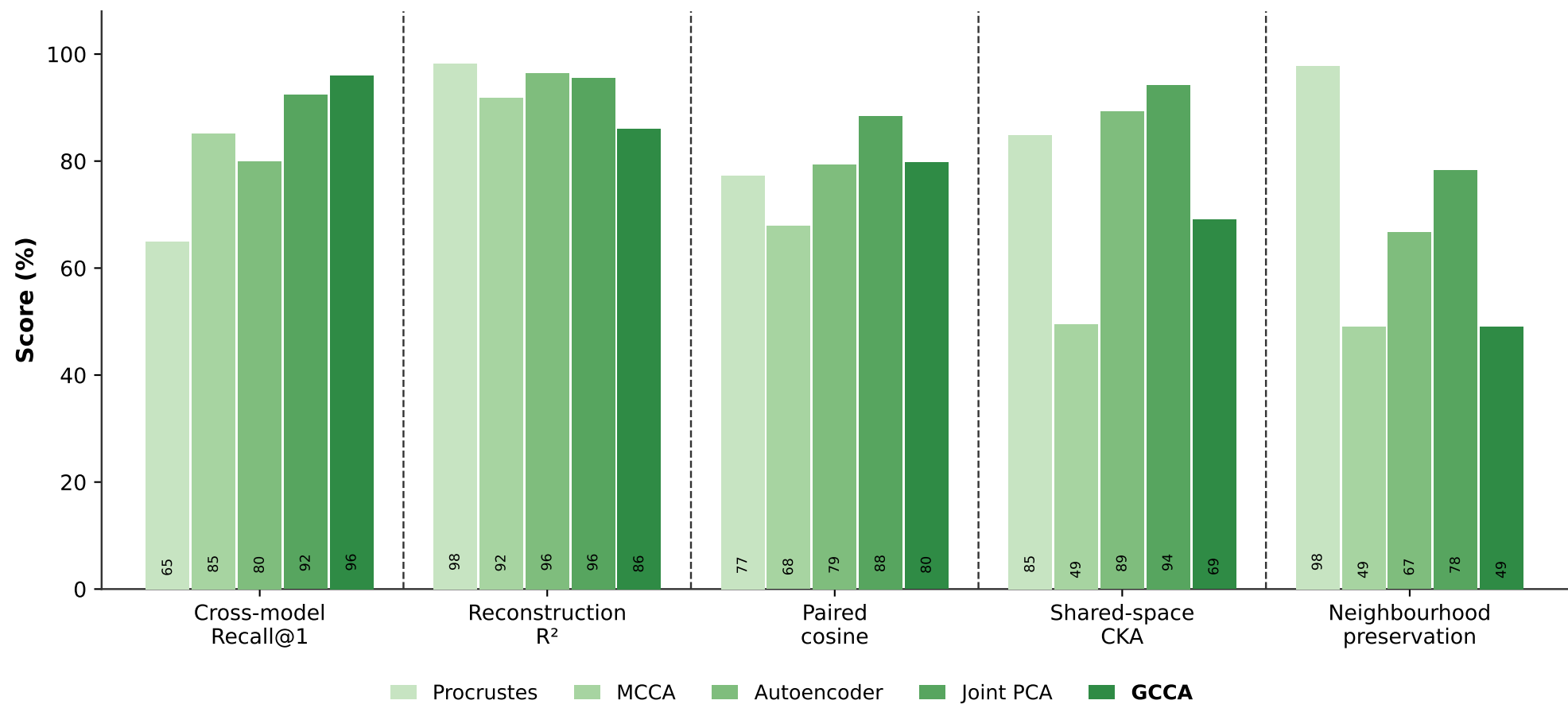
Alignment methods — CPTAC · 5× · 512px (CONCH v1 / v1.5)
