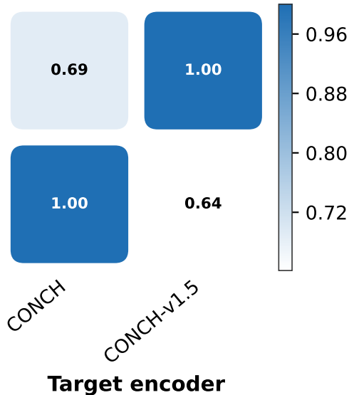
Retrieval Recall@1
