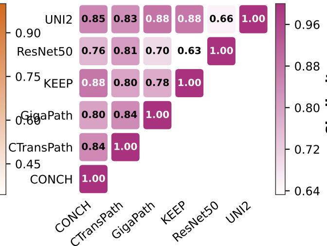
Distance Correlation
