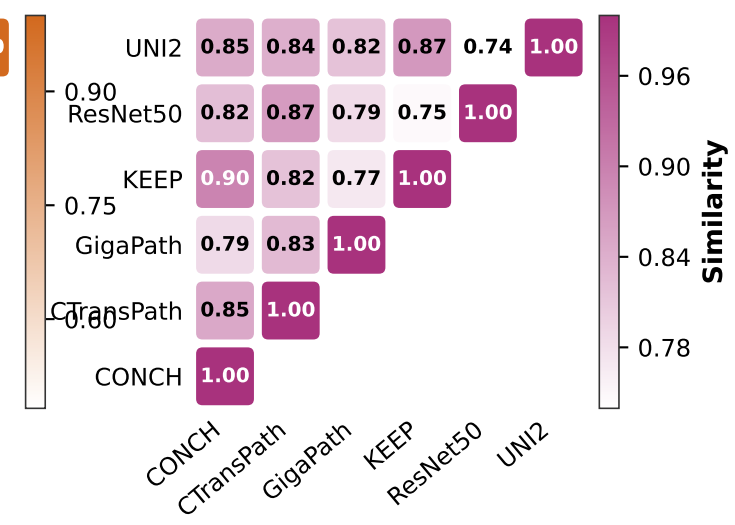
Distance Correlation
