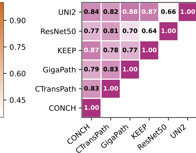
Distance Correlation
