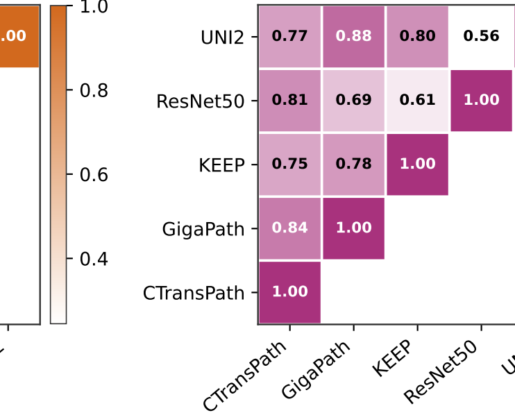
Distance Correlation
