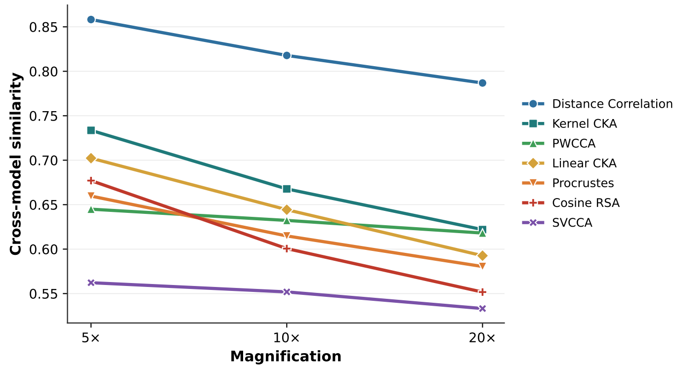
Agreement vs magnification — master_benchmark_256px
