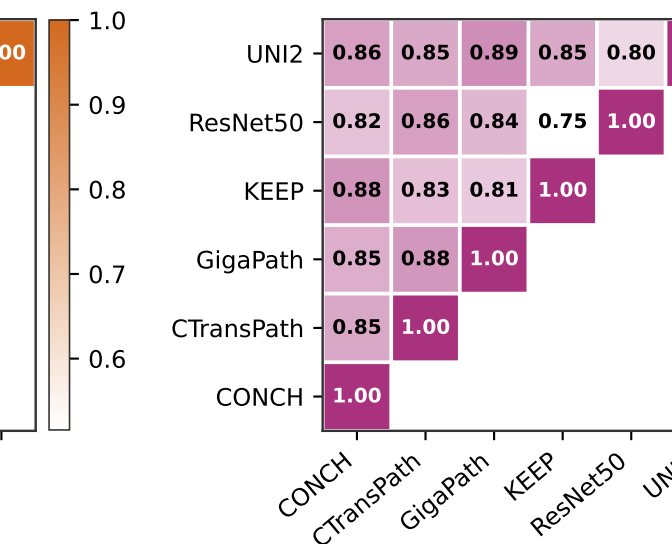
Distance Correlation
