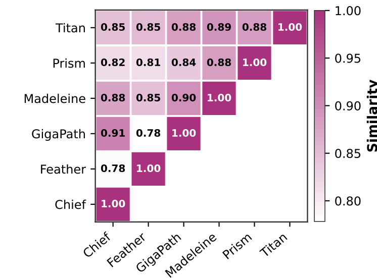
Distance Correlation
