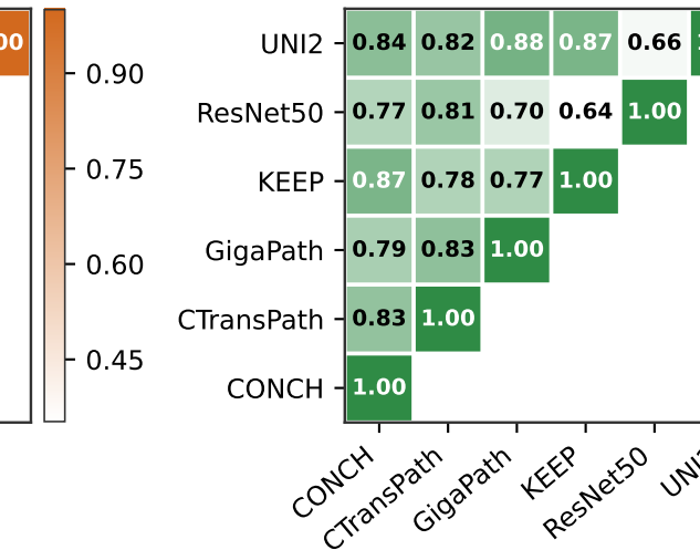
Distance Corr.
