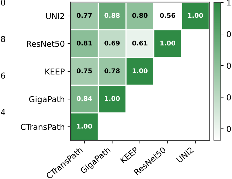
Distance Corr.
