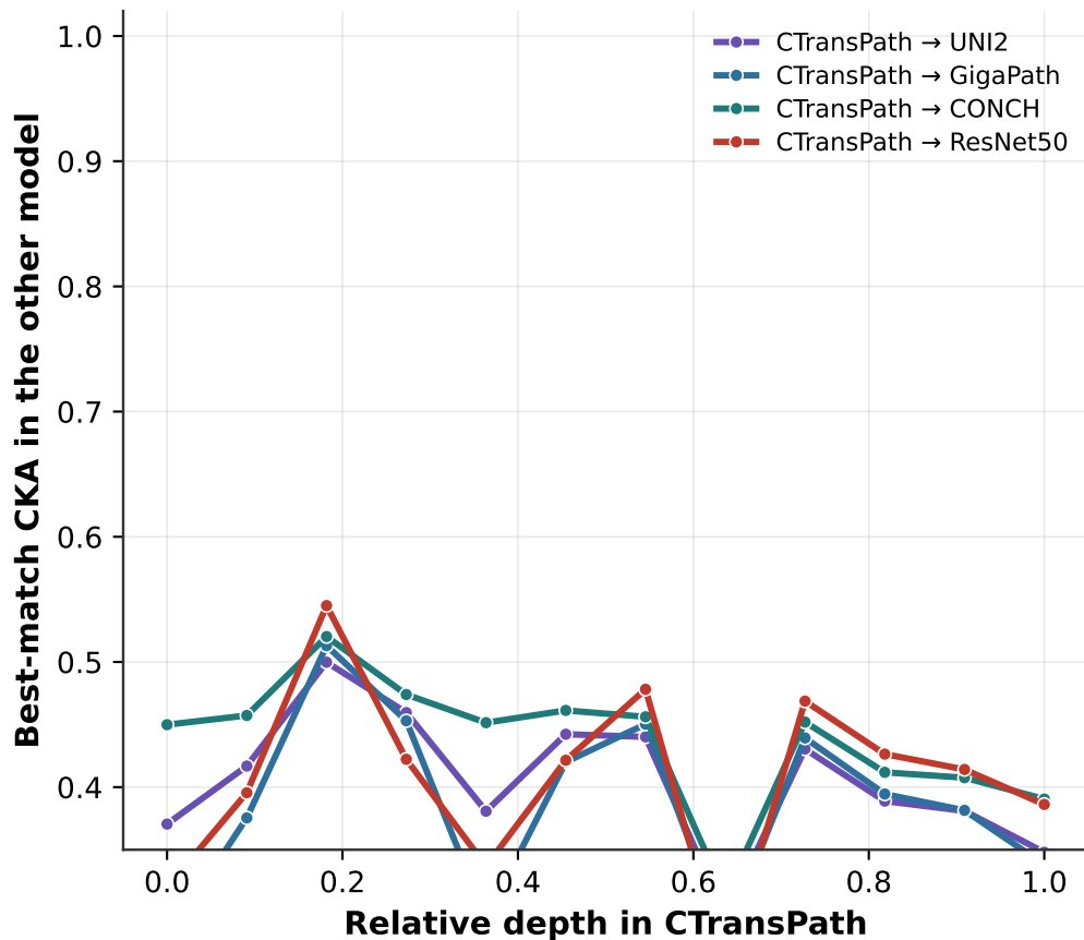
CTransPath's alignment across depth
