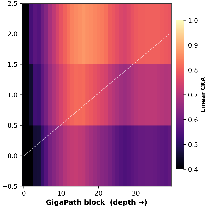
Block-by-block CKA
