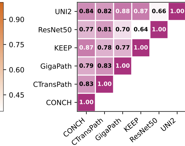
Distance Correlation
