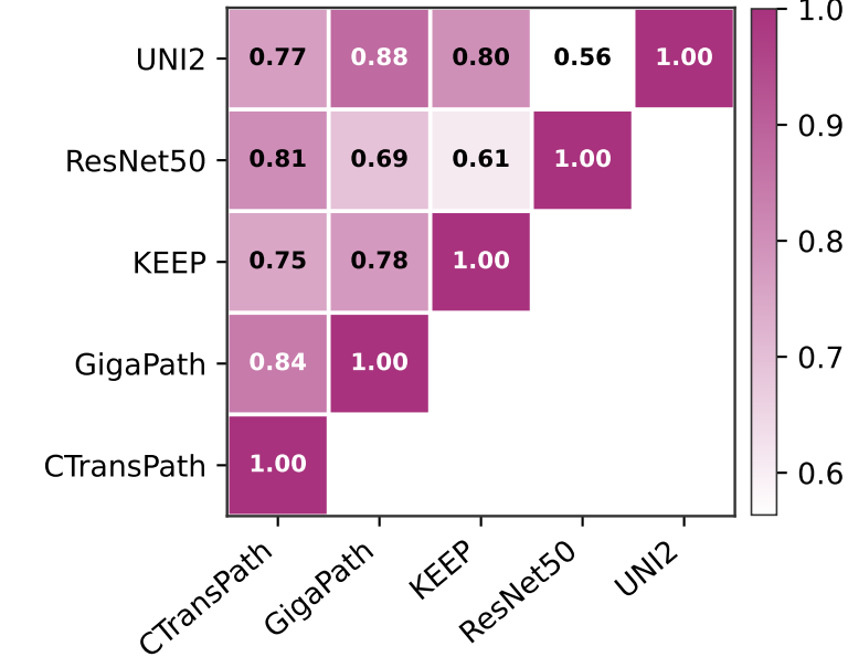
Distance Correlation
