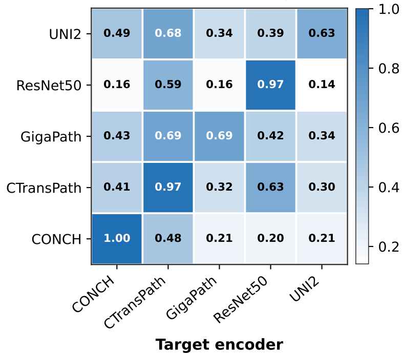
Retrieval Recall@1
