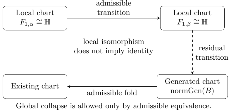
Figure 1: Local closure does not imply global collapse. A solid arrow denotes an admissible transition as described in Section 7; a dashed arrow denotes a residual transition as described in Section 8. The generated chart is normalized rather than collapsed, reflecting the Gen-normalization procedure of Section 11.
