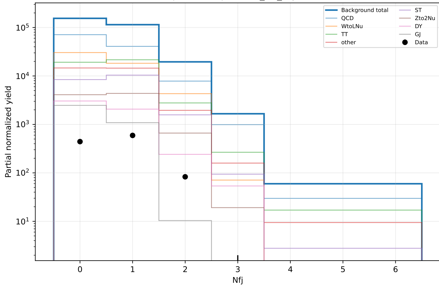
Partial preview nfj in cat7_SR_highDeltaM
