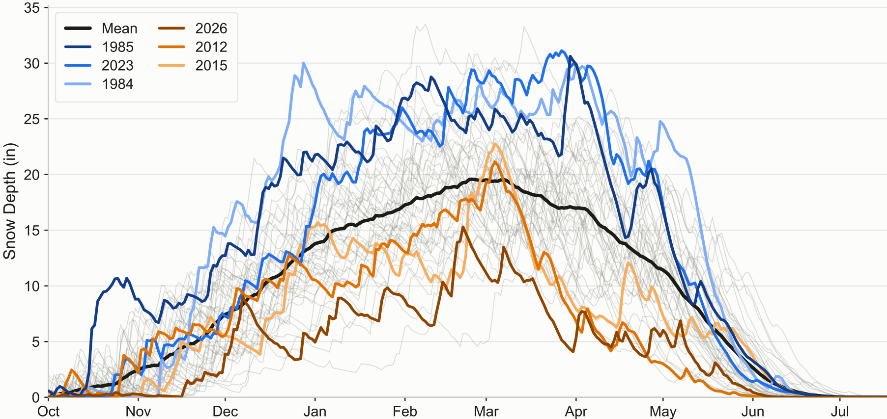
Colorado Rocky Mountains Snow Depth ERA5 (1981–2026)
