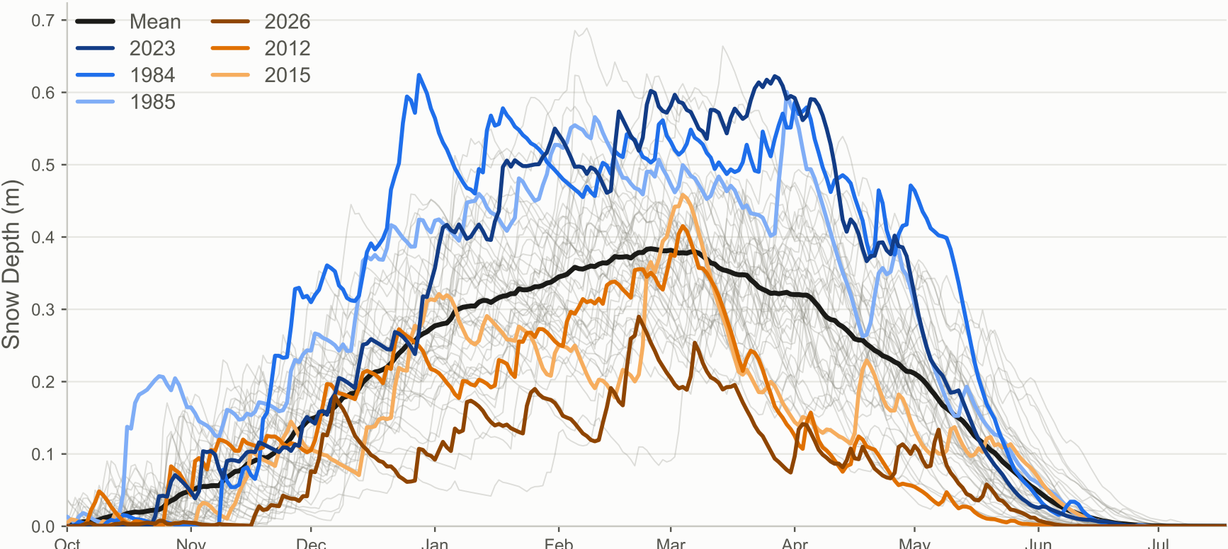
Colorado Snow Depth by Water Year, ERA5 (1981–2026)
