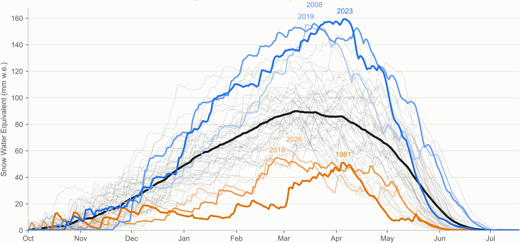
Colorado Snow Water Equivalent by Water Year, ERA5 (1981–2026)
