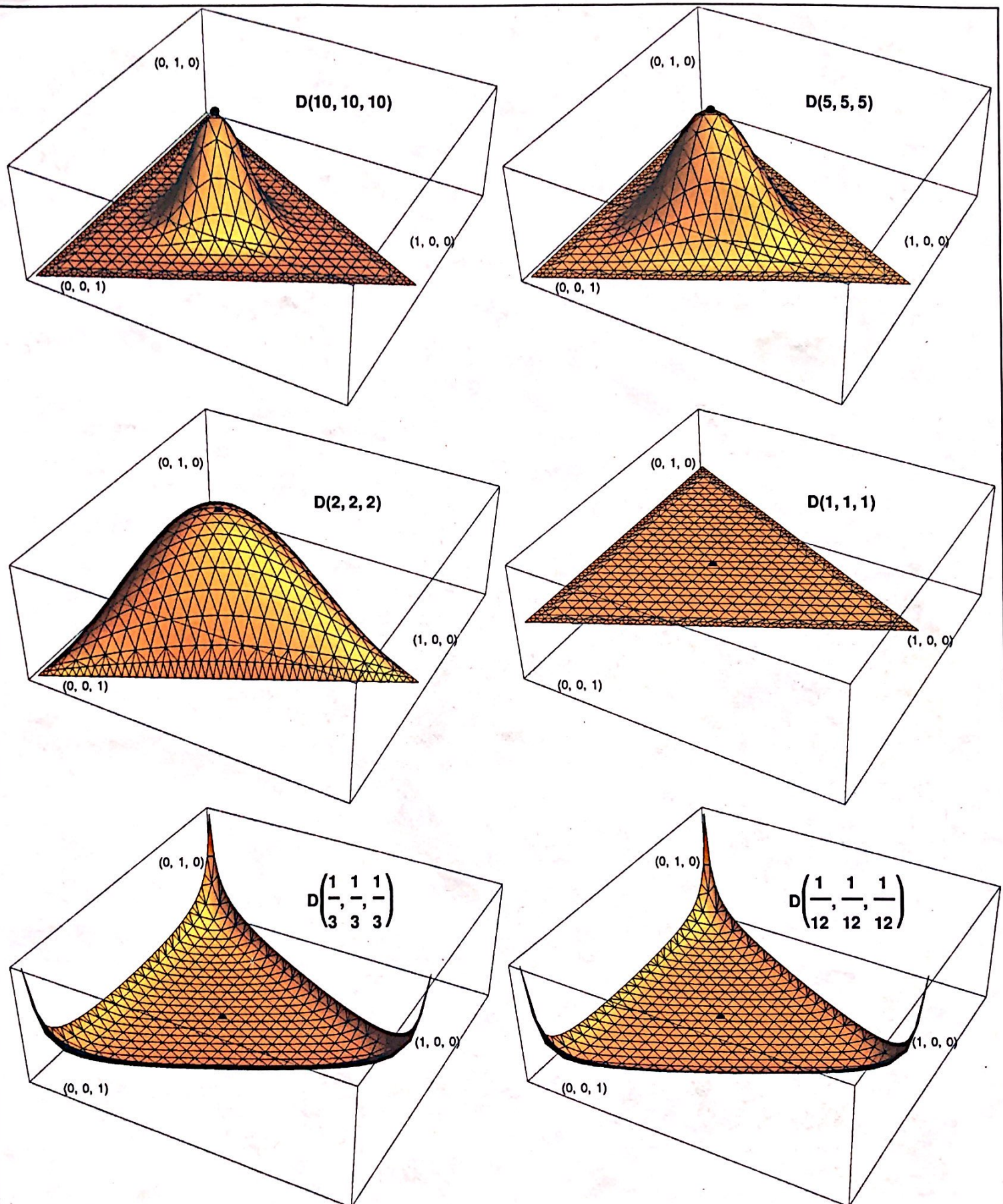
Figure 2. Densities of symmetric 3-component Dirichlets, illustrating how shape changes with concentration. In each case, the mean is (1/3, 1/3, 1/3) (shown with a dot). (Simplex vertices are labeled nearby; vertical scaling varies by plot, precluding comparison of density values across plots.)
