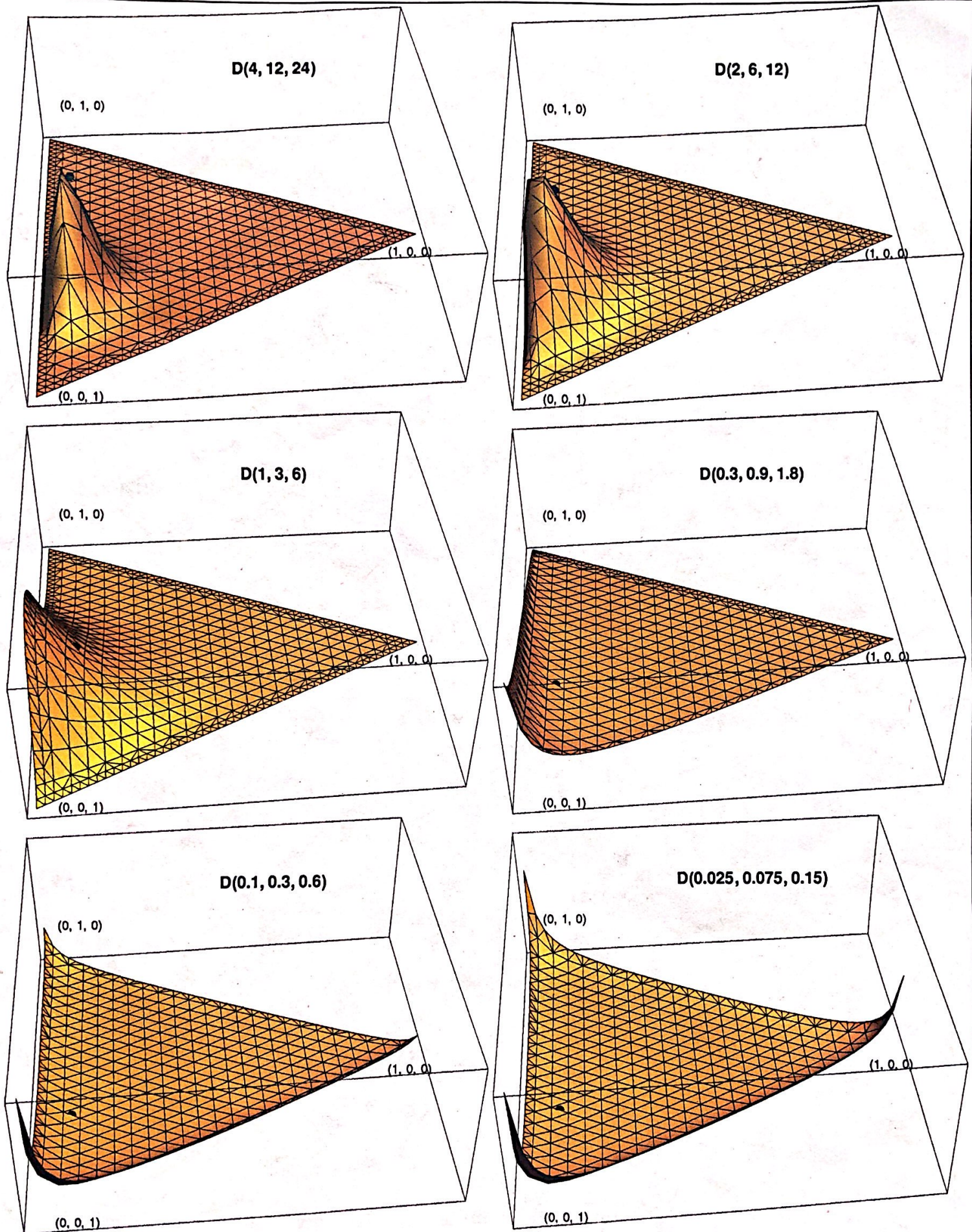
Figure 3. Densities of asymmetric 3-component Dirichlets; in each case, the mean is (0.1, 0.3, 0.6) (shown with a dot). (Vertical scaling varies by plot.)
