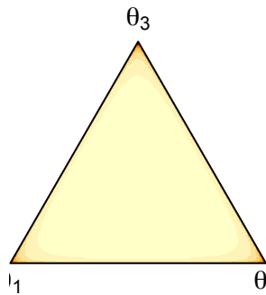
Dirichlet(0.7,0.7,0.7)
