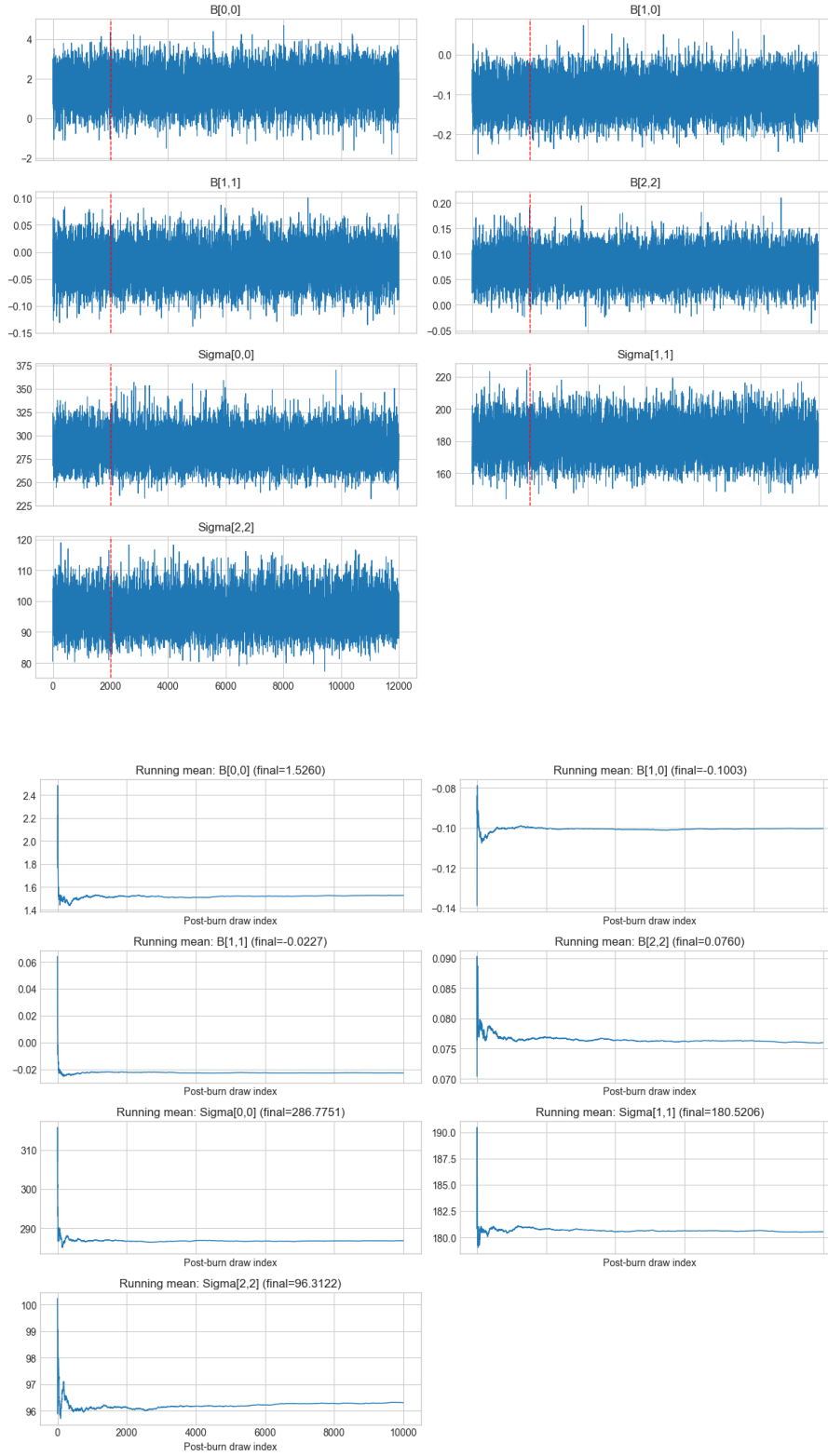
Figure 7: Trace plot and running posterior mean of intercept and lag-1 oil production coefficient, and reduced-form innovation
