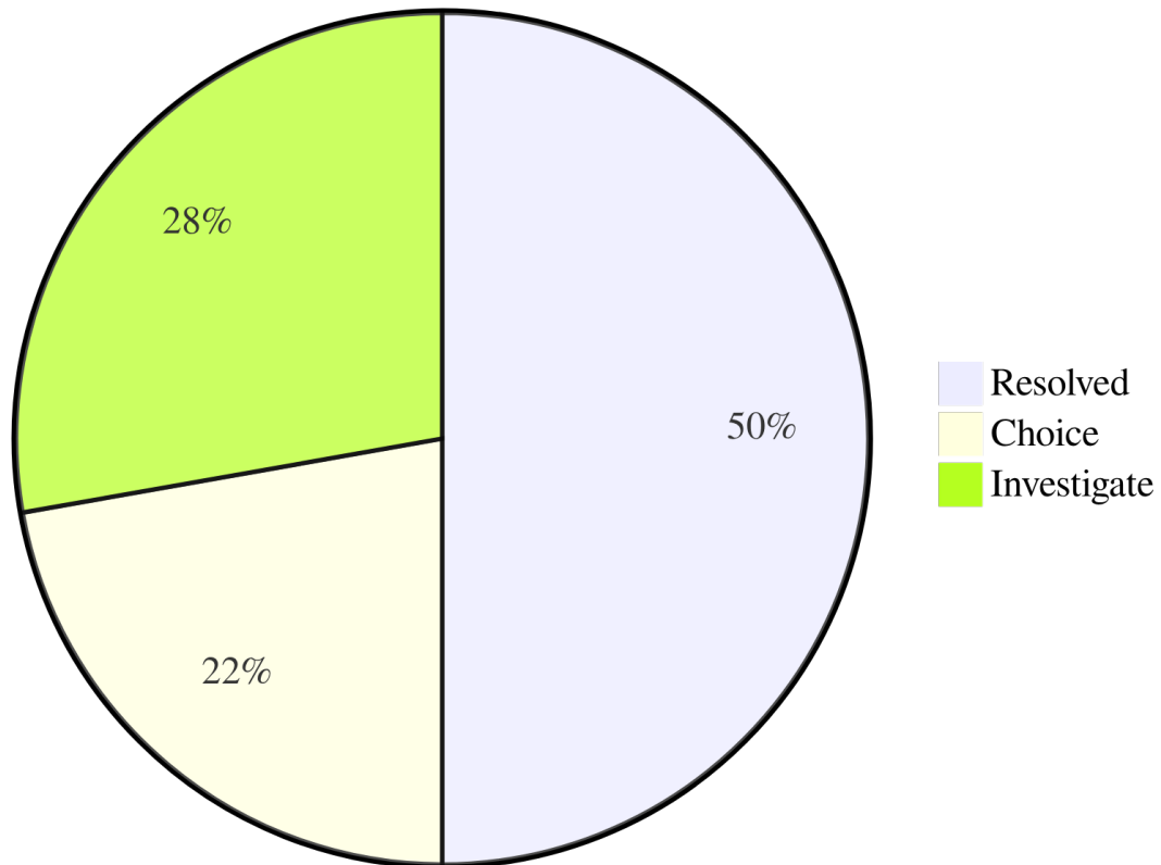
Open-question statuses
