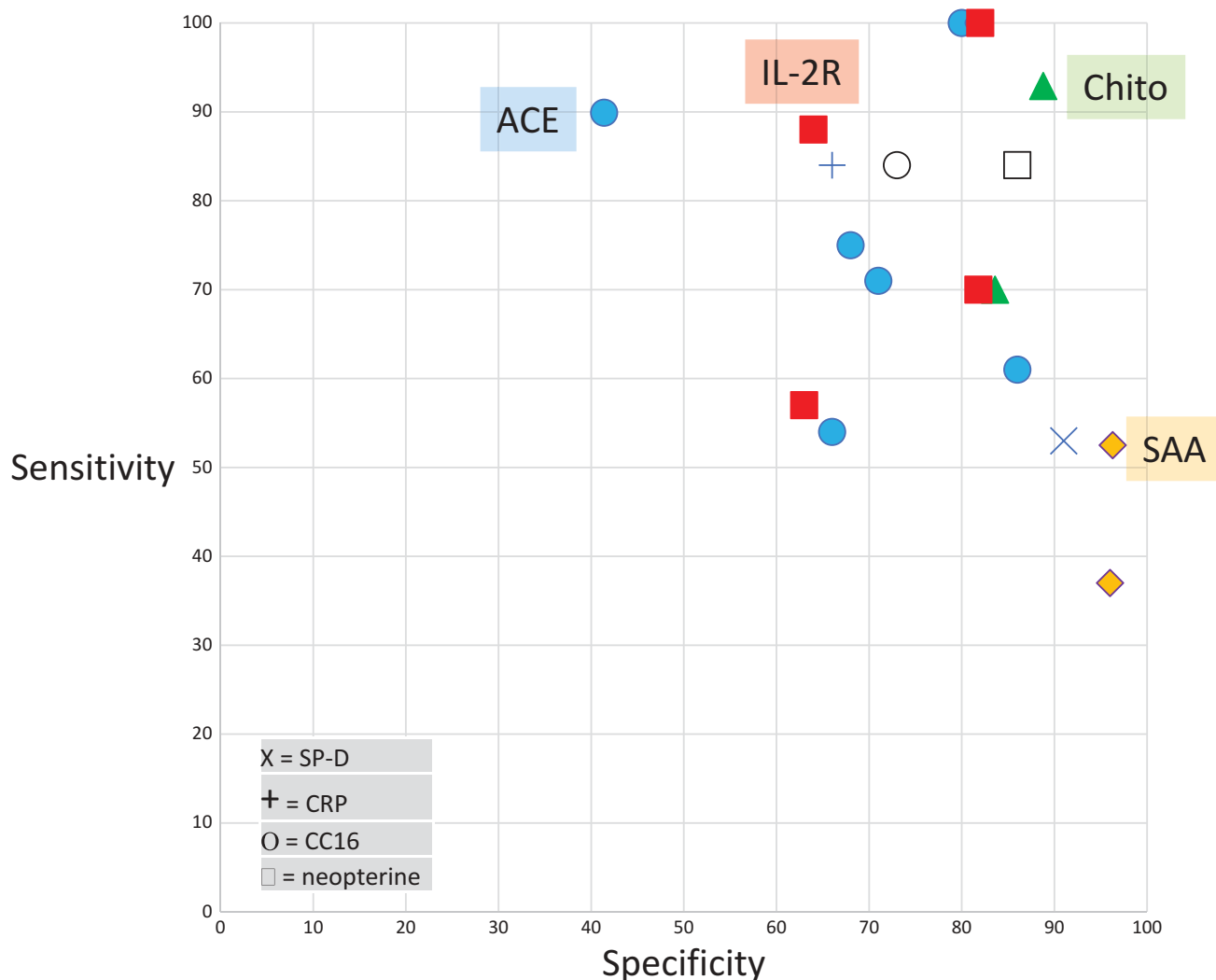
Figure 1. Sensitivity (SE), specificity (SP), positive predictive values (PPV) and negative predictive values (NPV) in studies testing different biomarkers in patients with unselected sarcoidosis.
