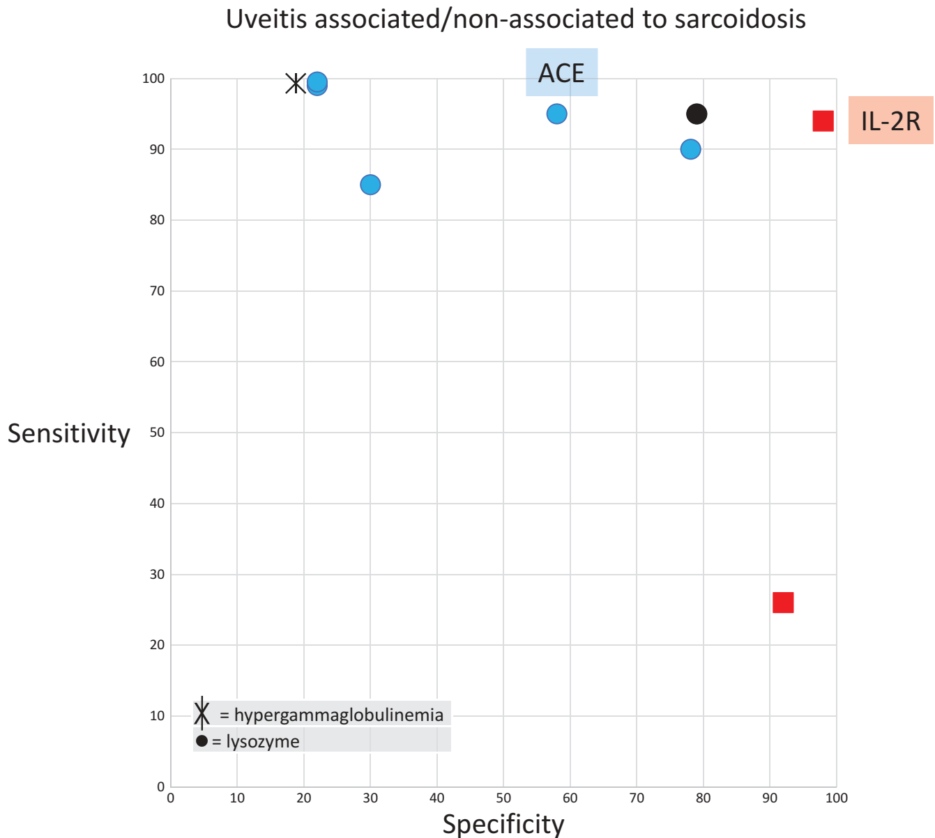
Figure 2. Sensitivity (SE), specificity (SP), positive predictive values (PPV) and negative predictive values (NPV) in studies testing different biomarkers in patients with ocular sarcoidosis.
