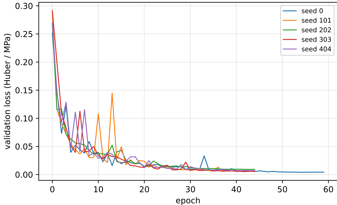
Phase-1 Deep Ensemble — validation loss per member
