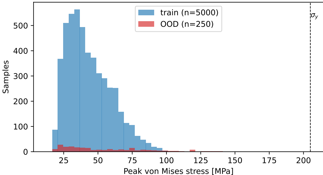
Peak stress distribution across the sweep
