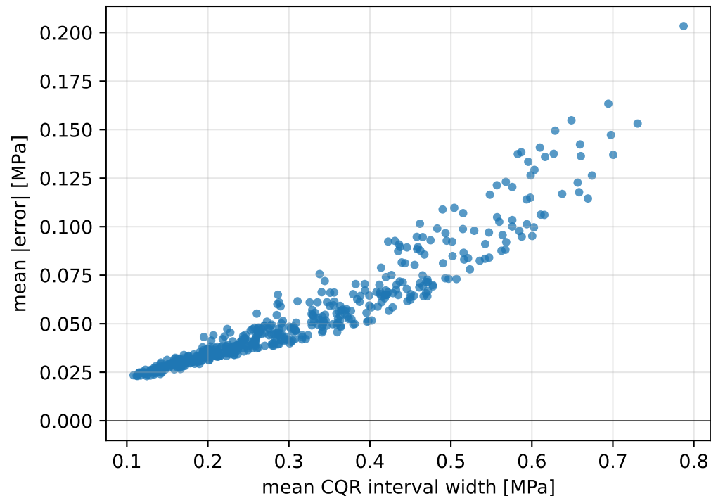
Phase-2: CQR width vs. error (Pearson 0.944)
