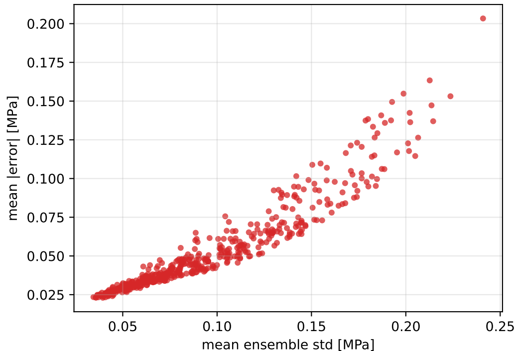
Phase-1: ensemble std vs. error (Pearson 0.944)
