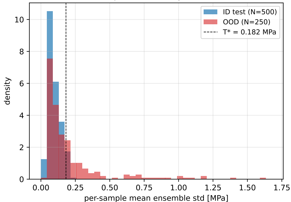
Per-sample uncertainty: ID vs OOD
