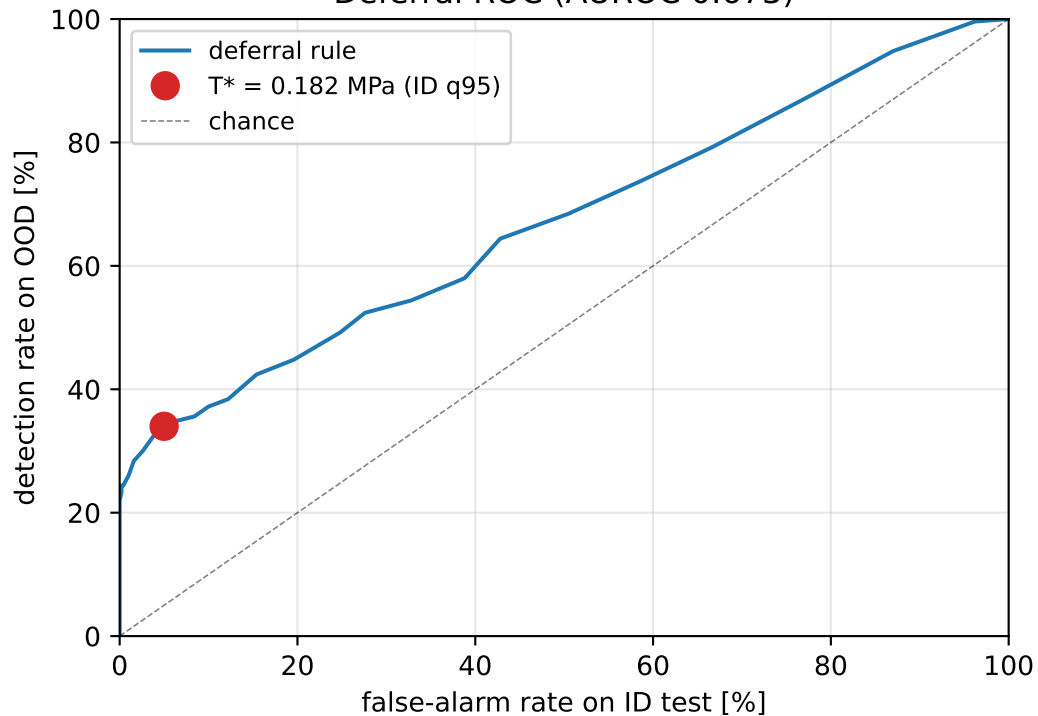
Deferral ROC (AUROC 0.673)
