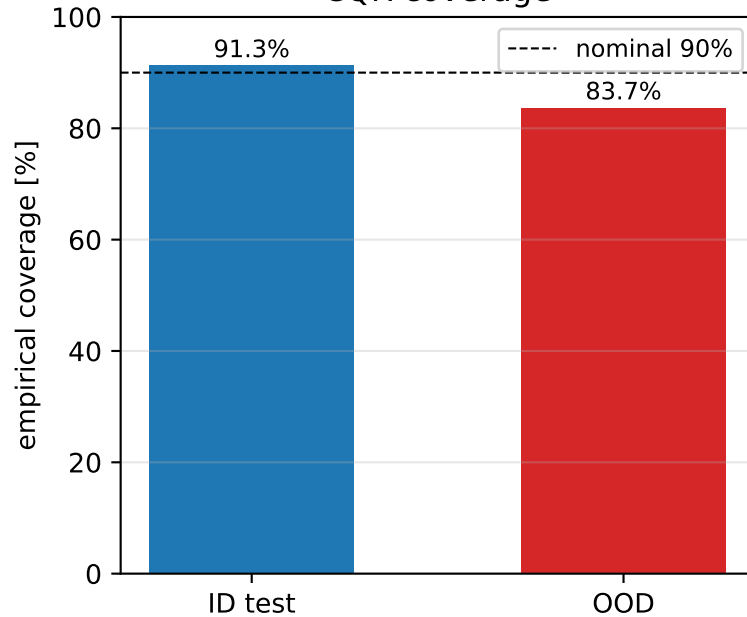
CQR coverage
