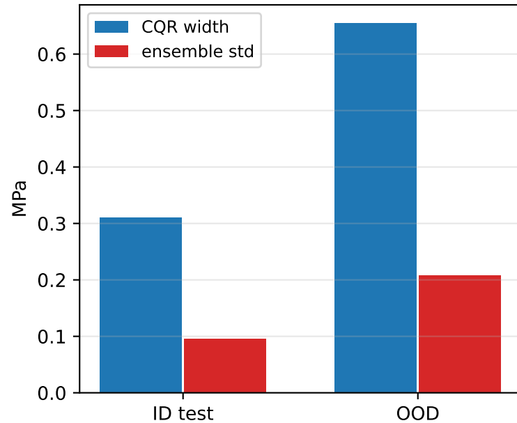
Uncertainty scale
