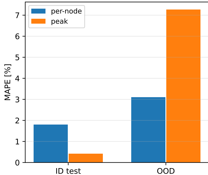
Accuracy
