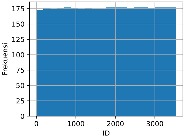
Histogram ID
