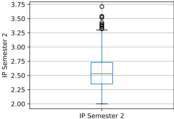
Boxplot IP Semester 2
