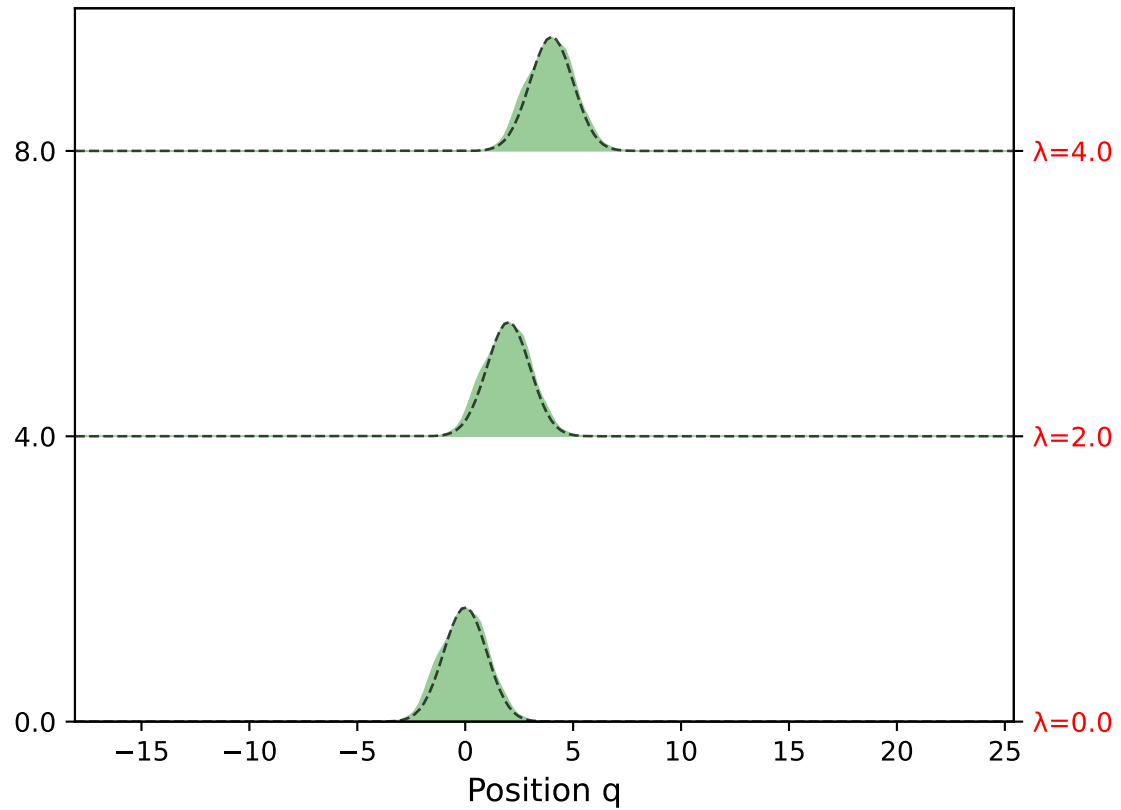
CD-HMC - Gaussian Moving Mean
