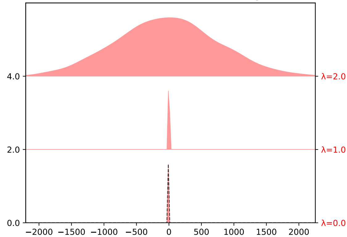
CD-HMC - Gaussian Annealing
