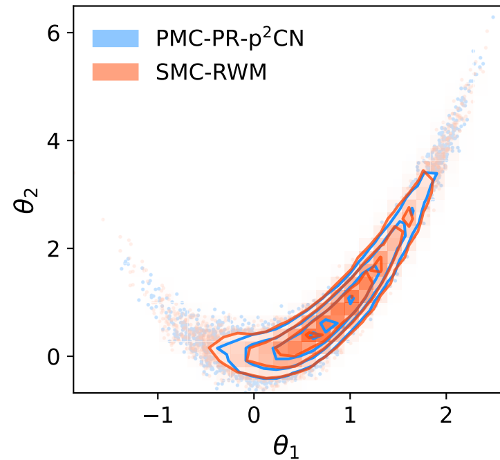
Rosenbrock-10
