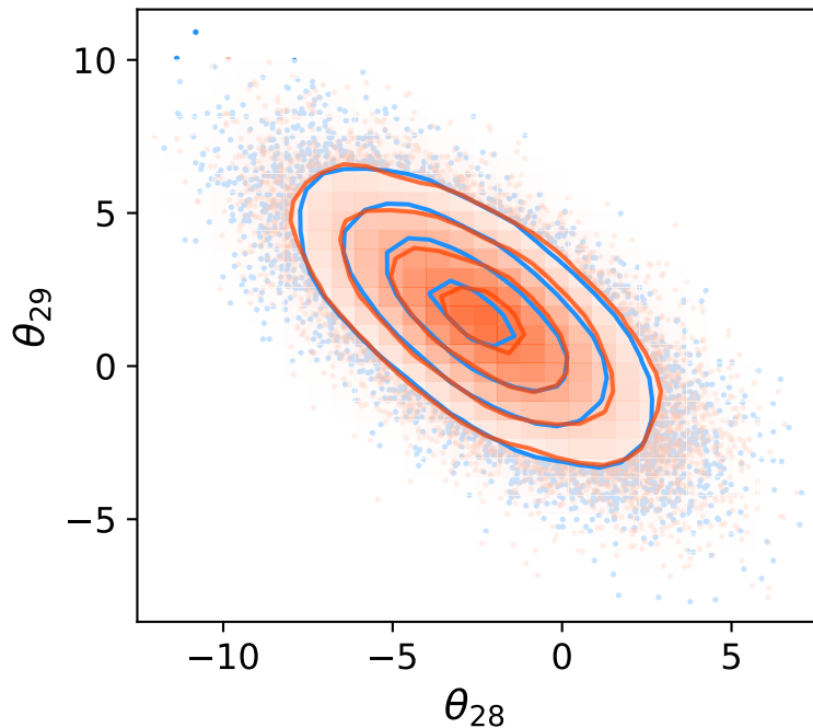
Sonar-61
