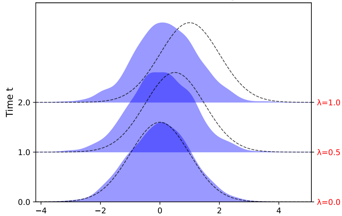
CD-HMC - Gaussian Moving Mean
