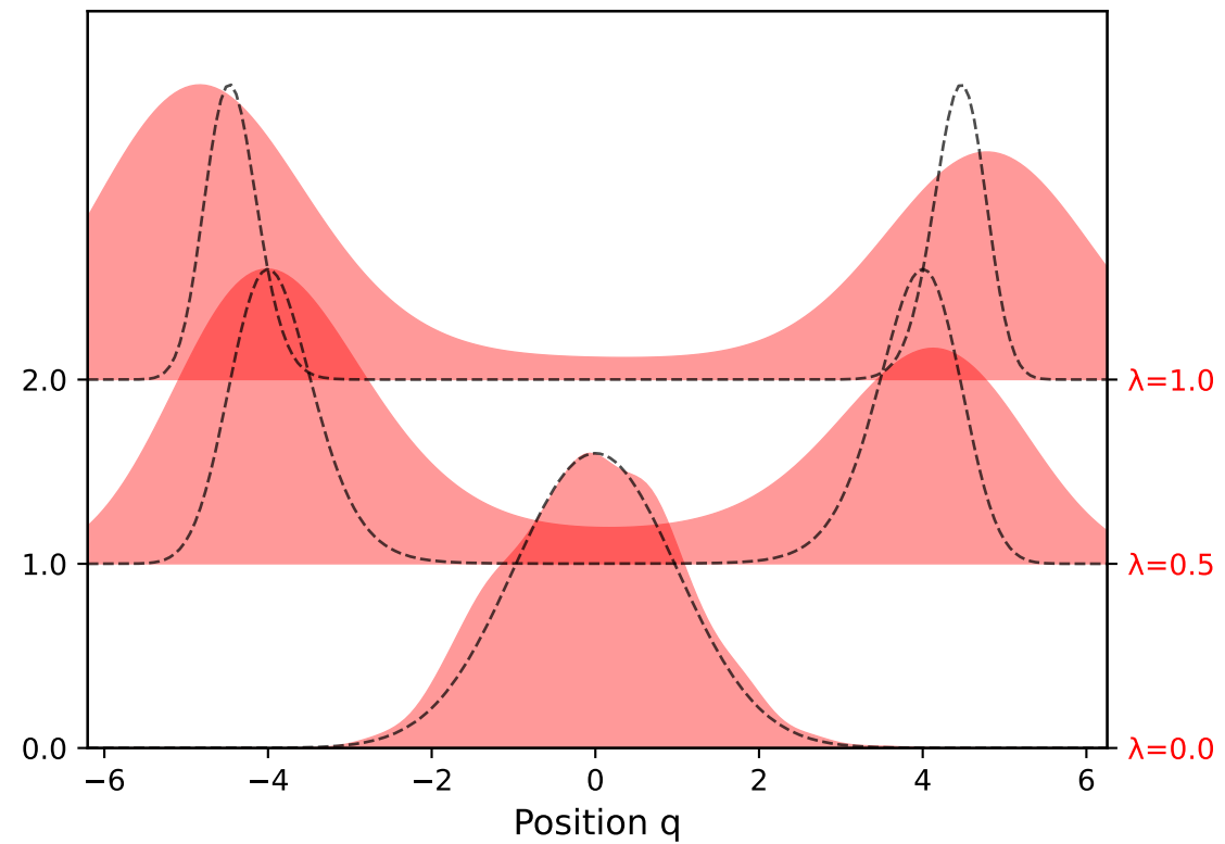
CD-HMC - Double Well
