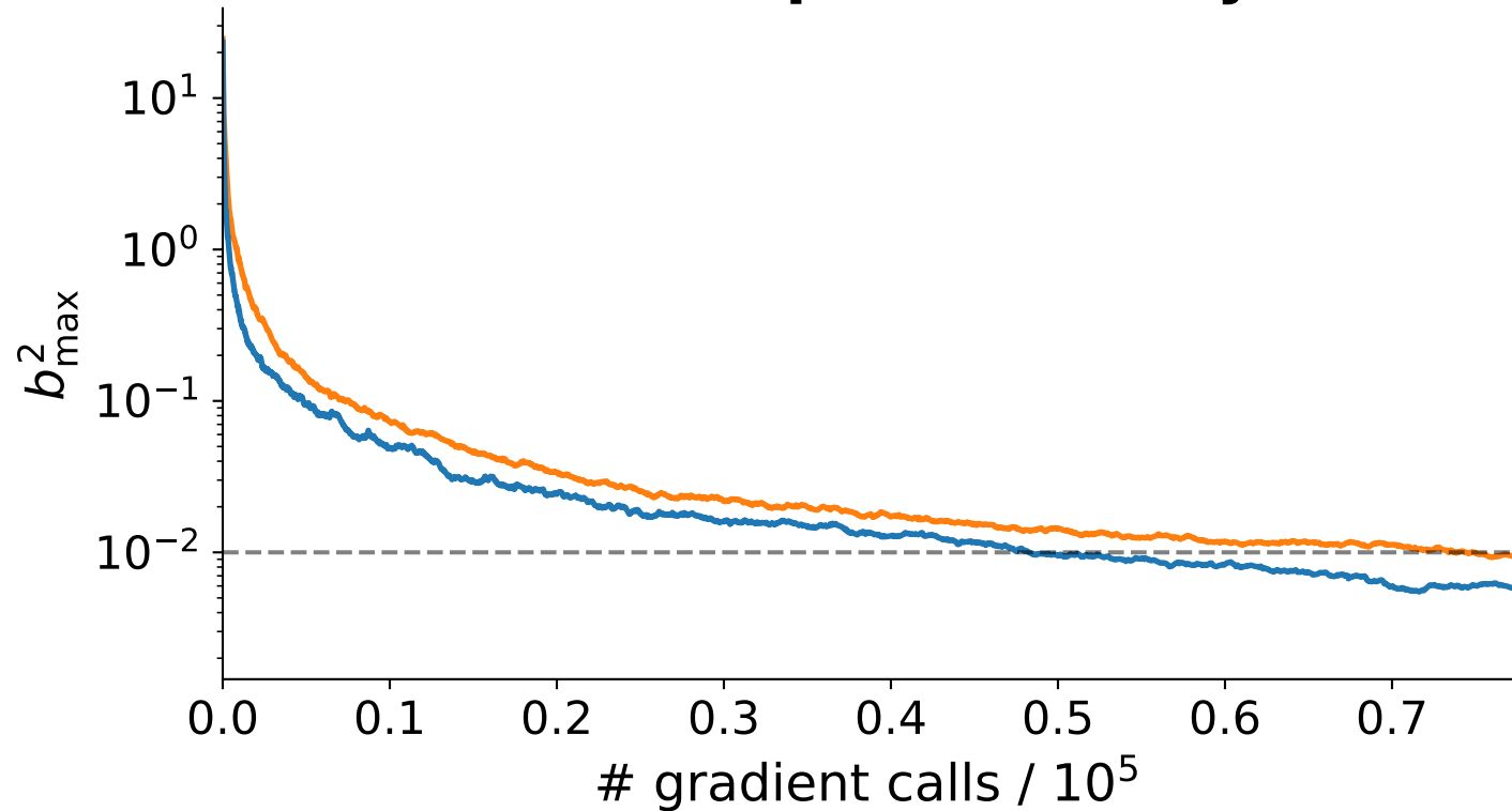
Item Response Theory
