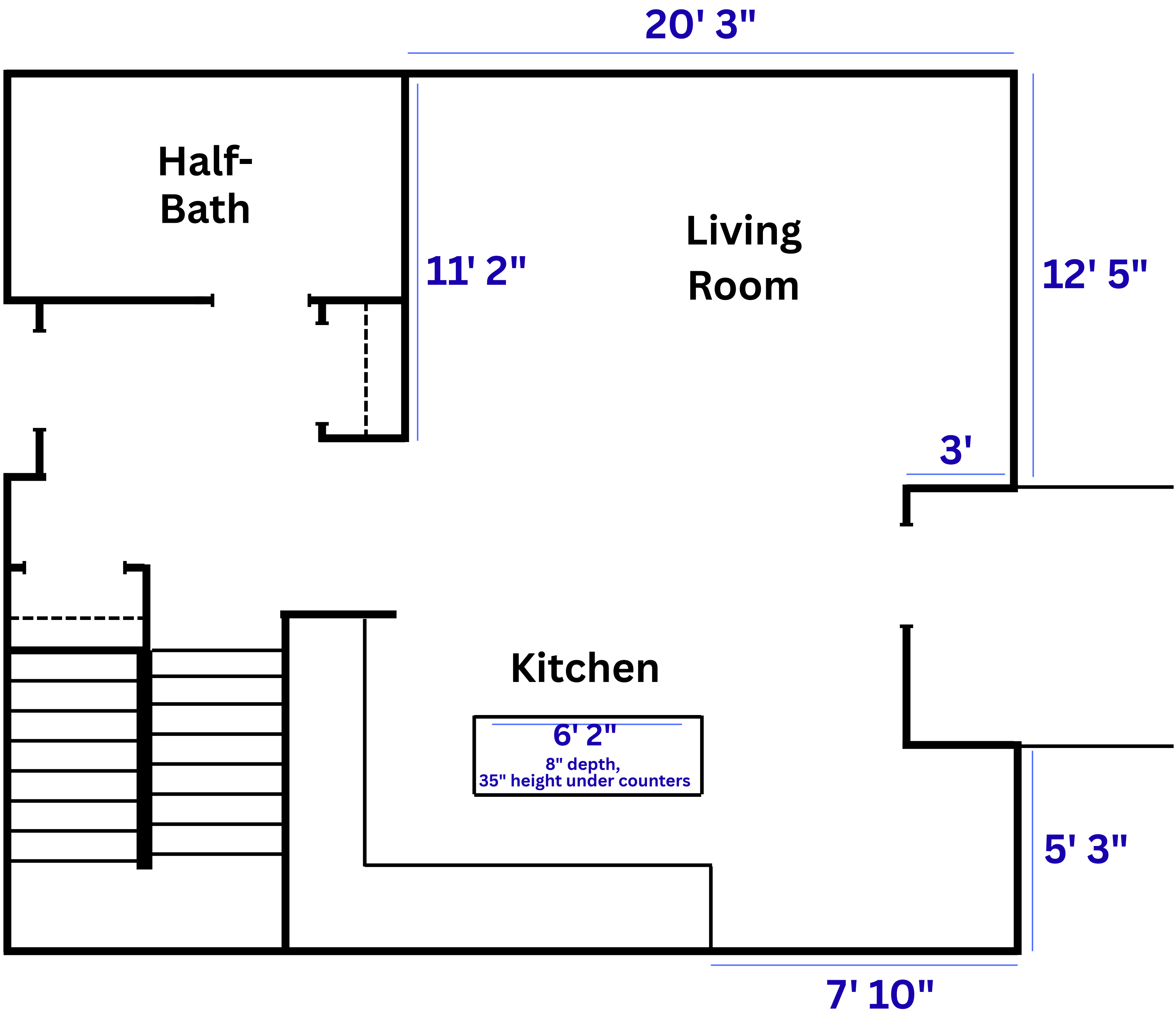
FIRST FLOOR
