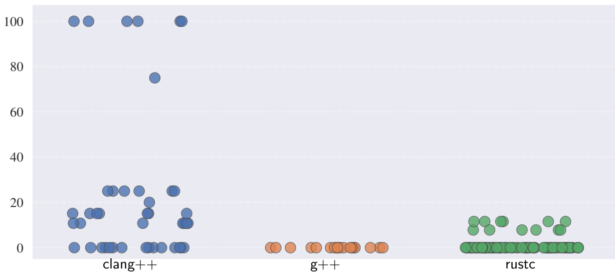
Fortified Functions (%)
