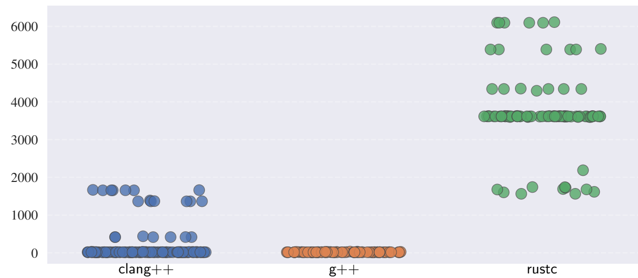
Fortified Functions (%)
